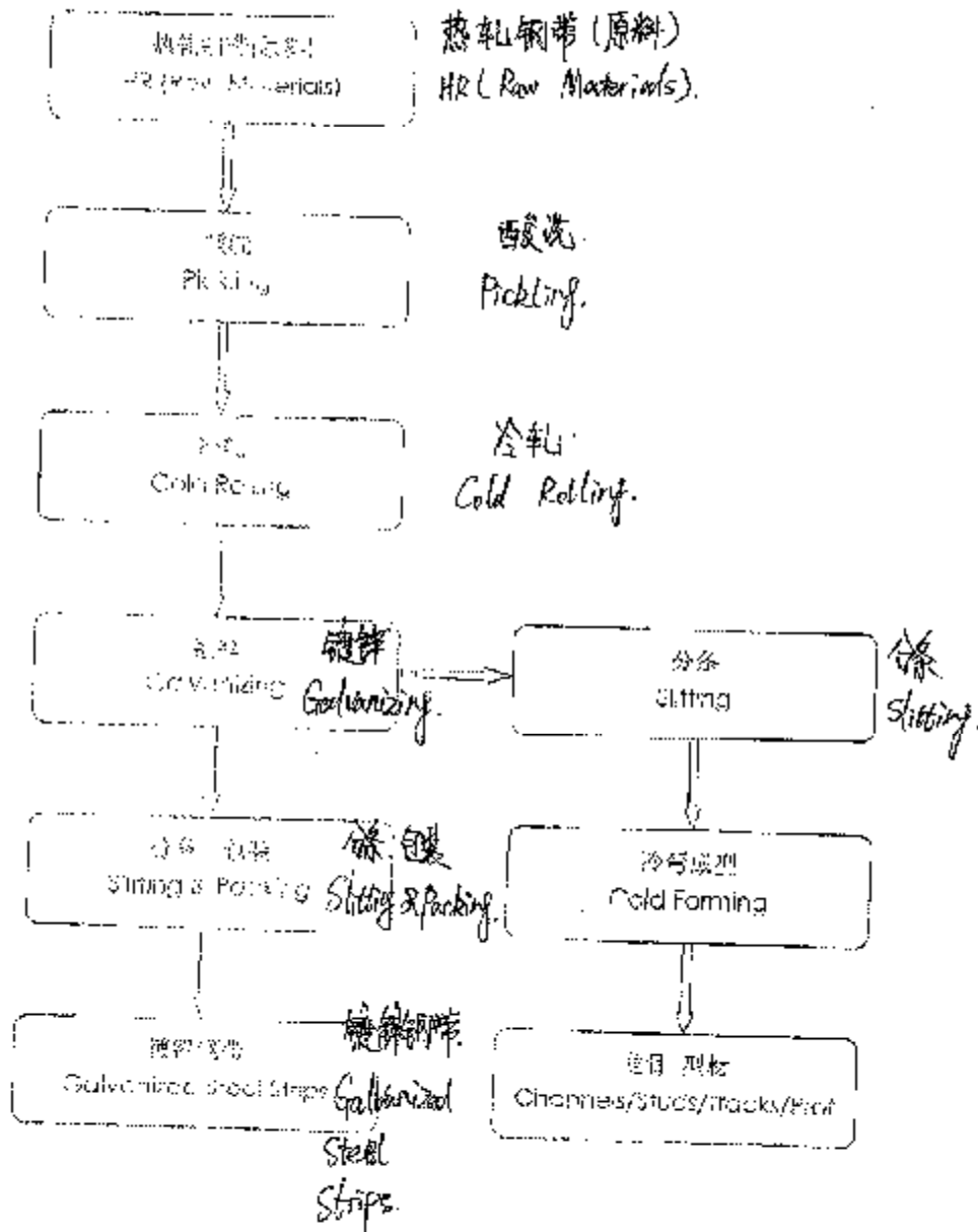
Flow Chart of Hot Dipped Galvanized Steel Strips in Coils and Steel Profiles
