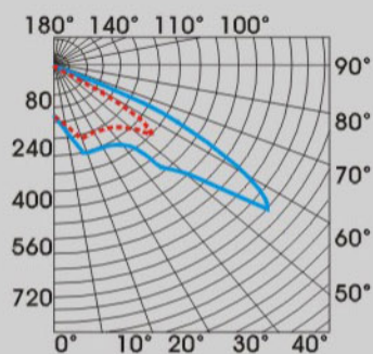
配光曲线: Luminous intensity curve
