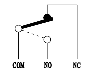
SCHMATIC
