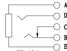
ST-194 SCHEMATIC
