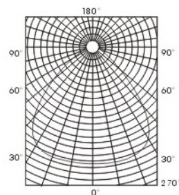
配光曲线: Luminous intensity curve
