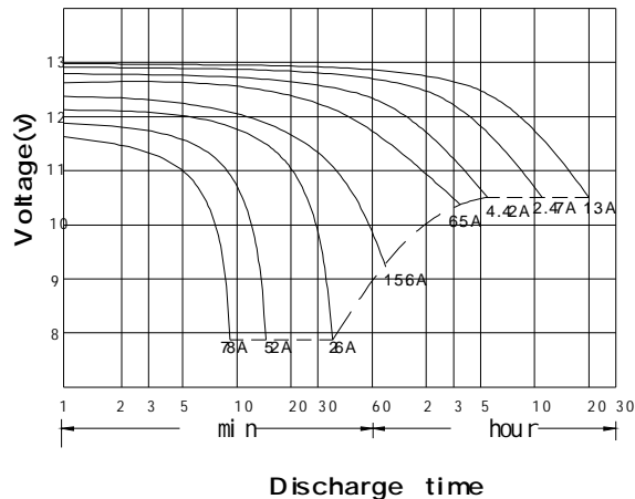
Discharge time vs. discharge current (25°C, 77°F)
