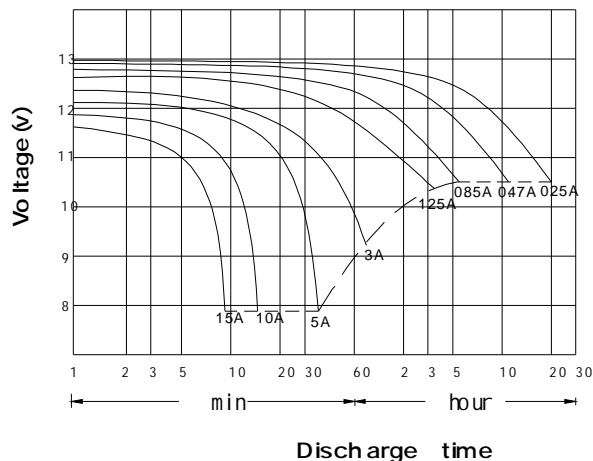
Discharge time vs. discharge current(25°C,77 °F)
