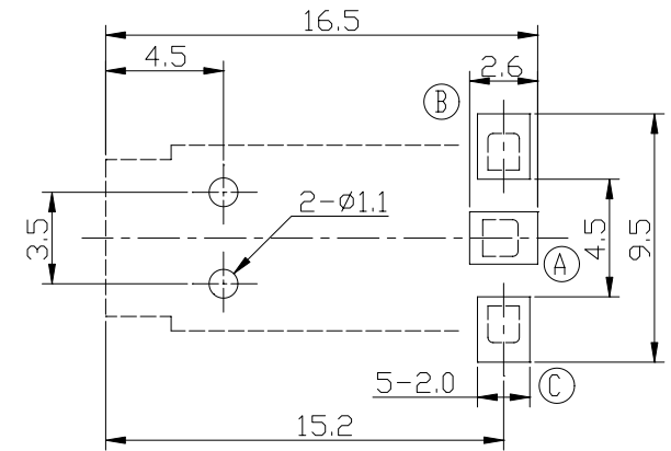
PCB HOLE & SURFACE MOUNT LAYOUT
