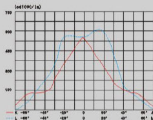
配光曲线: Luminous intensity curve
