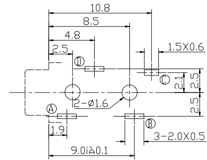
PC BOARD HOLE LAYOUT
