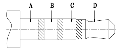
Ø 2.5 MATE PLUG
