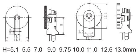
Plastic Wheel(90 teeth and 18 teeth) 塑料轉輪(90齒和18齒)
