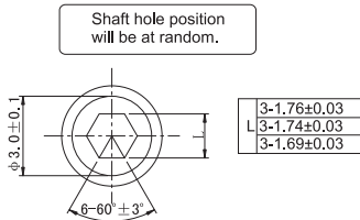
Shaft hole shape and dimension 軸孔外形尺寸
