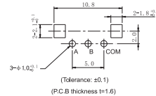
P.C.B.mounting hole detail
