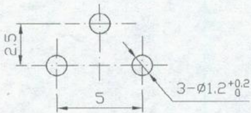
PCB TERMINAL POSITION
