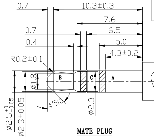
ST-201B SCHEMATIC
