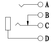
ST-201 SCHEMATIC
