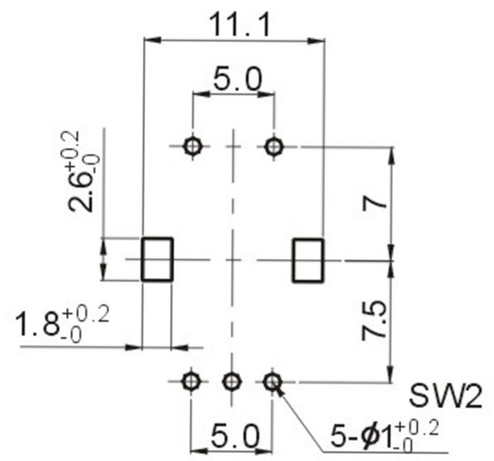
P.C.B. MOUNTING DETAIL
