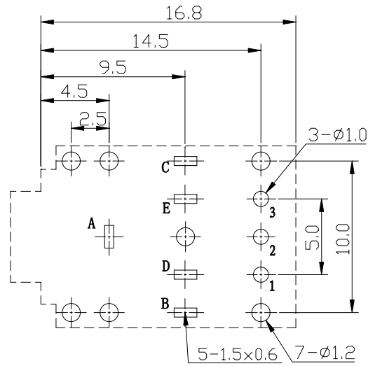
HOLE LAYOUT (BOTTOM VIEW)
